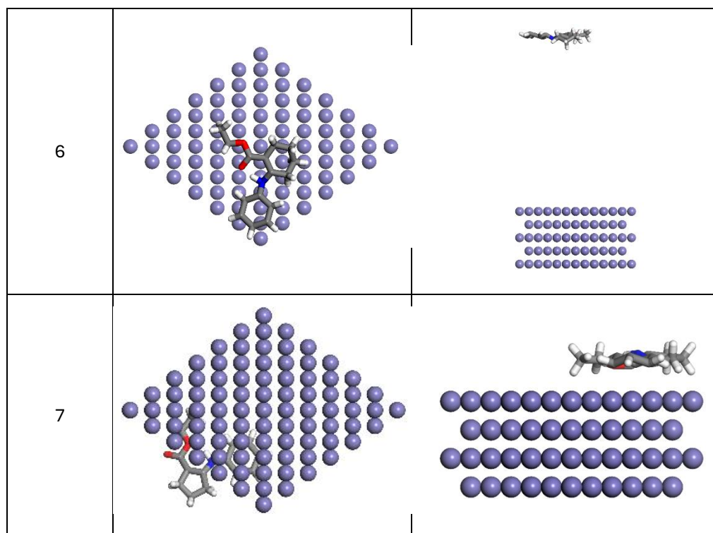
Figure 2: Global minimum adsorption configurations of enamine derivatives (L1–L7) on the Fe(110) surface obtained from Monte Carlo simulations: (A) Top views and (B) Side views
