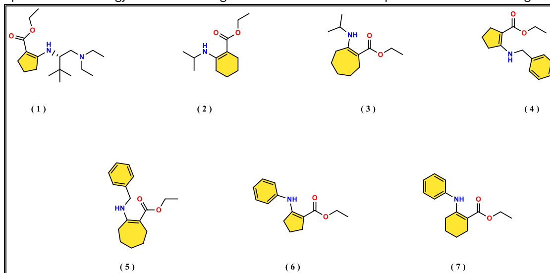
Figure 1: 2D chemical structures of the studied enamine derivatives (L1 – L7).
